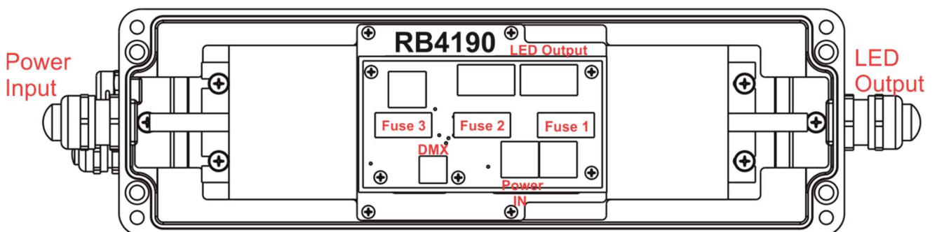
Connection points
