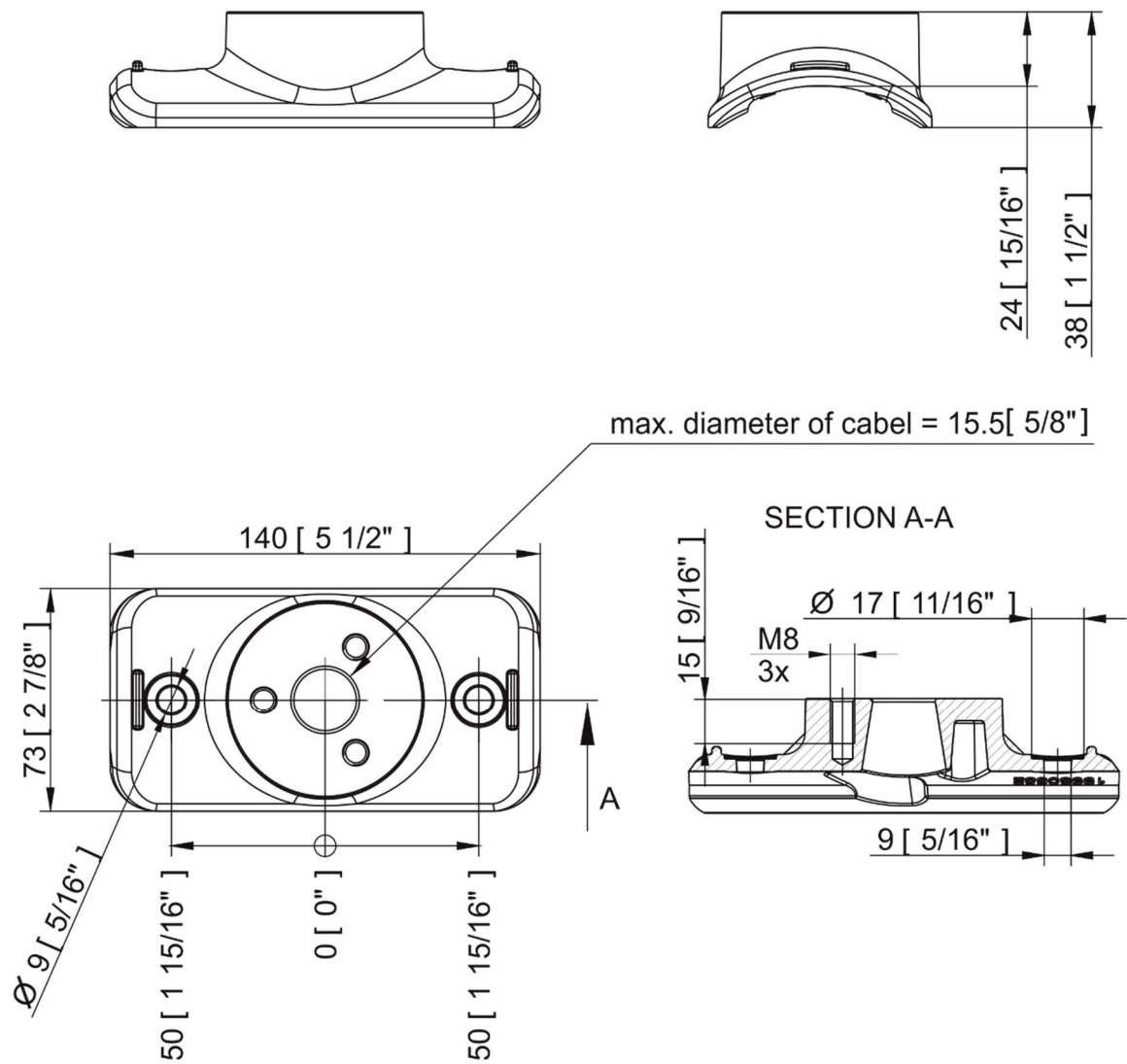
Pole clamp adaptor for Calumma
