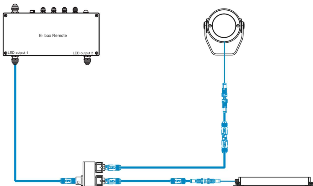
T-connector MID 05 (P/N 13054130)
