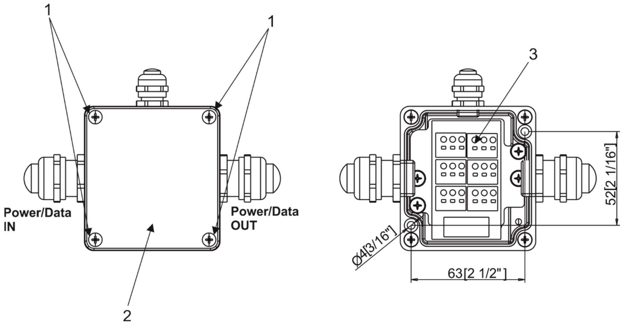
Junction box with four outputs
