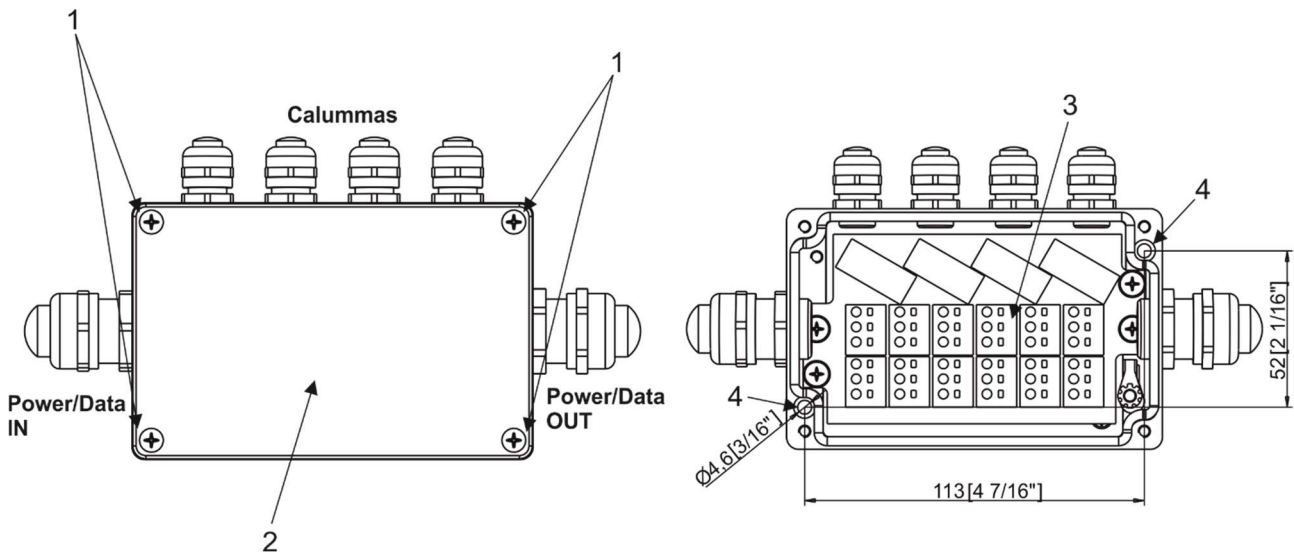
Junction box with four outputs
