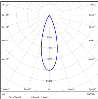
Calumma L SC RGBW 6500K 30dg
