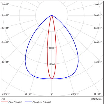
Calumma L SC RGBW 6500K 15x90dg
