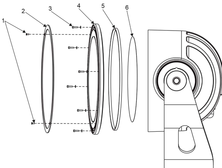
DETAIL A
