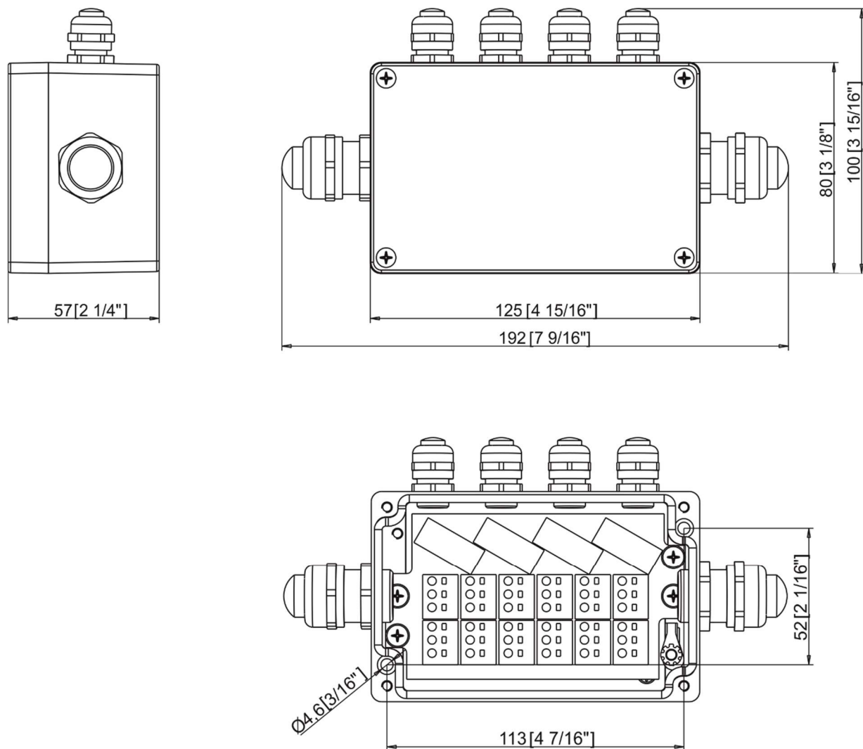
Junction box with four outputs
