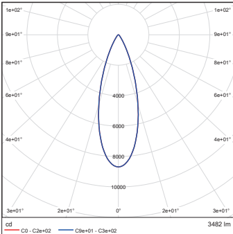
Eminere Remote MC 4 RGBCW 35dg
