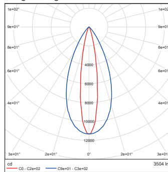
Eminere Remote MC 4 RGBCW 15dg x 45dg
