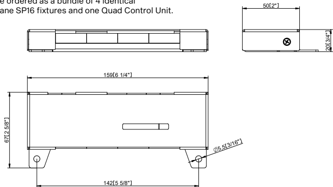
Quad Control Unit dimensions (CE Only)
