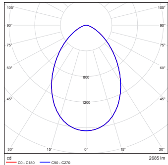
Ambiane AP RGBNW 67dg; with Frosted glass; without Anti-Glare ring
