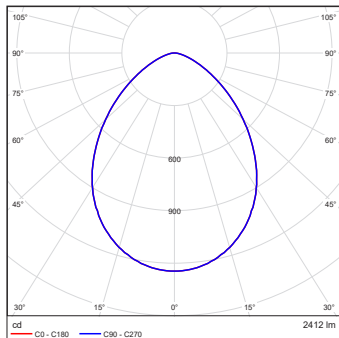
Ambiane AP RGBNW 80dg; with Frosted glass; without Antiglare ring
