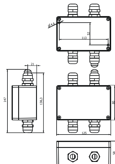
Junction box
