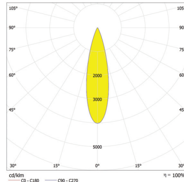
ArcSource Outdoor 24MC - 26° 350mA
