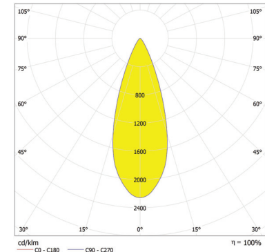
ArcSource Outdoor 24MC - 36° 350mA
