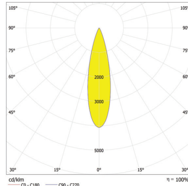
ArcSource Outdoor 24MC - 26° 700mA
