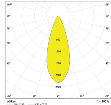
ArcSource Outdoor 24MC - 36° 700mA
