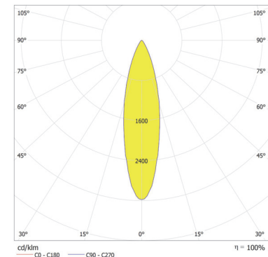
ArcLine Outdoor Double Optic 36 RGB - 26°
