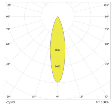
ArcLine Outdoor Double Optic 48 RGB - 26°
